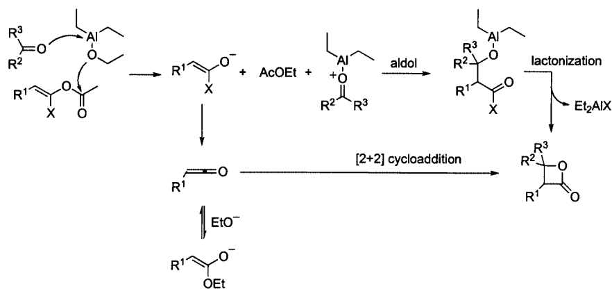
Scheme 4. Activation of the enol acetate by \text{Et}_2\text{AlOEt} .
