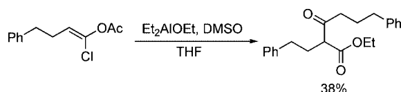
Scheme 6. Claisen condensation.
