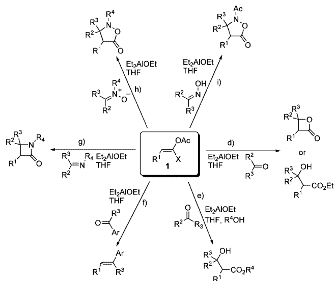
Scheme 3. Reactivities of \alpha -haloenol acetates with electrophiles.
