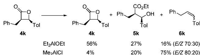
Scheme 5. Decarboxylation of 2-oxetanones promoted by \text{Et}_2\text{AlOEt} and \text{Me}_2\text{AlCl} .
