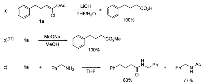
Scheme 2. Reactivities of \alpha -haloenol acetates with nucleophiles.
